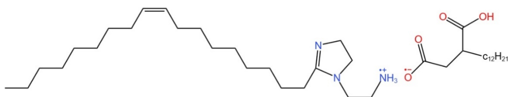
Heptadecenyl imidazoline succinate
